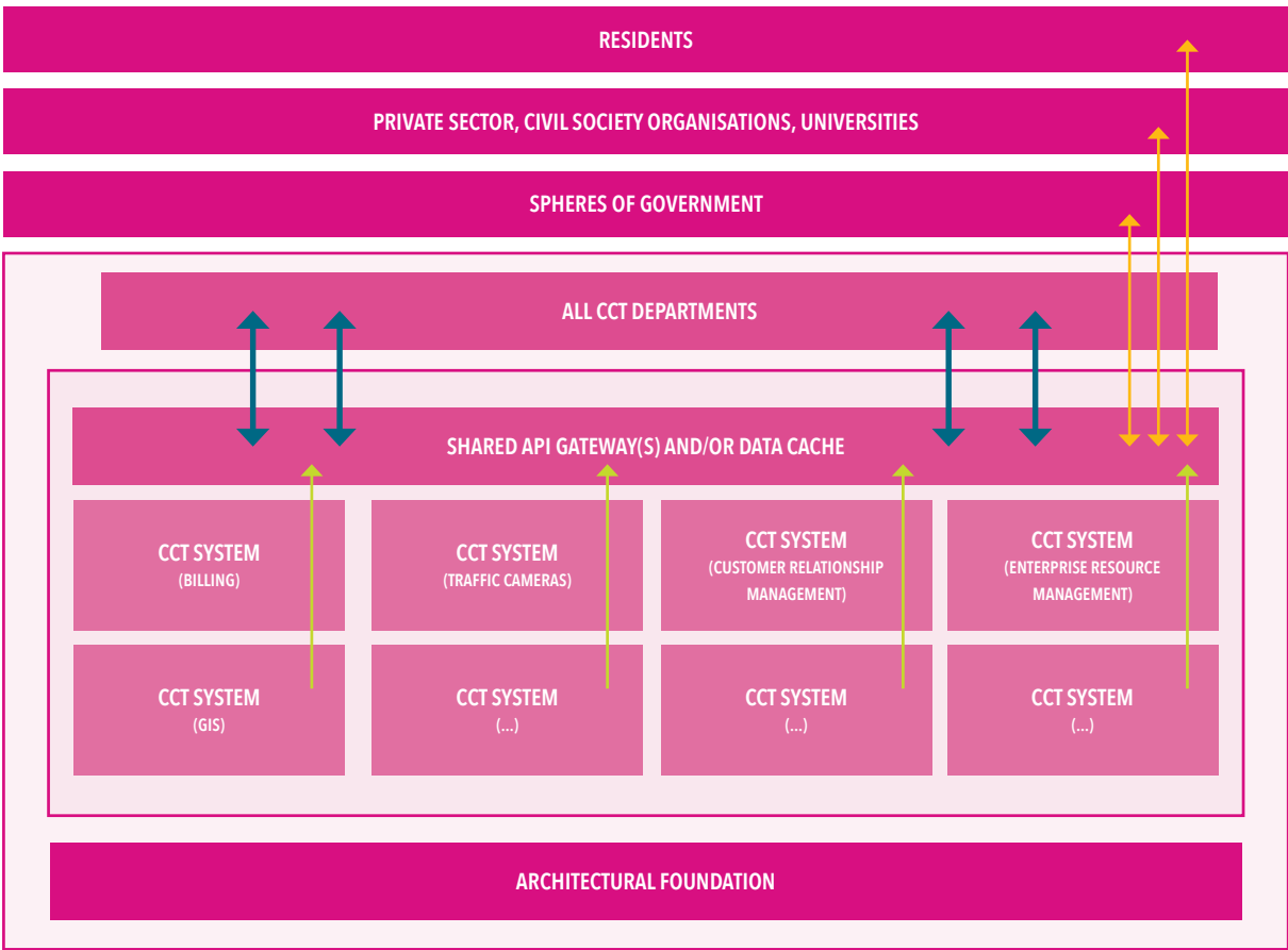
FIGURE 2: CCT AS A DATA ECOSYSTEM
